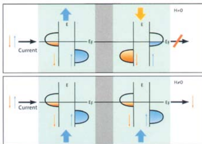
Fig. 9: Illustration of the magnetoresistance effect for a half-metal. Two ferromagnetic half-metallic layers (light green) separated by a non-magnetic metal (grey). In the absence of an external magnetic field ( H = 0 ) the two ferromagnets have antiparallel spin polarizations (blue and orange thick arrows at the top). In the presence of an external field ( H \neq 0 ) the two magnets have parallel spin polarization (two thick blue arrows at the bottom of the figure). As can be immediately understood, there will be no current for the upper case. For the lower case there will only be a spin down current.
