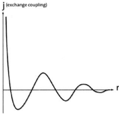
Fig. 5: Schematic illustration of the behaviour of the exchange coupling as a function of distance.
