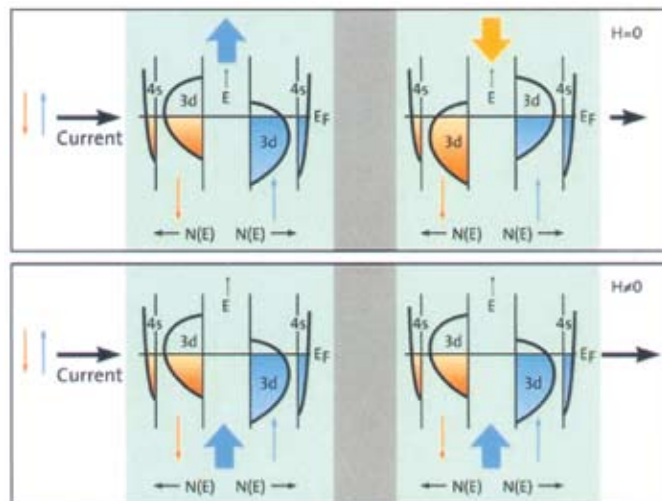
Fig. 6: Schematic illustration of the electronic structure of a trilayer system with two ferromagnetic layers (light green) on both sides separated by nonmagnetic material (grey). The top figure is for the case without external magnetic field ( H=0 ), i.e. when the two magnetic layers have opposite magnetizations (indicated by the thick blue and orange arrows at the top of the topmost figure). The bottom figure is for the case when an external magnetic field ( H \neq 0 ) has forced the two magnetizations to be parallel (two thick blue arrows at the bottom of the lower figure). The magnitude of the four magnetizations is the same.
