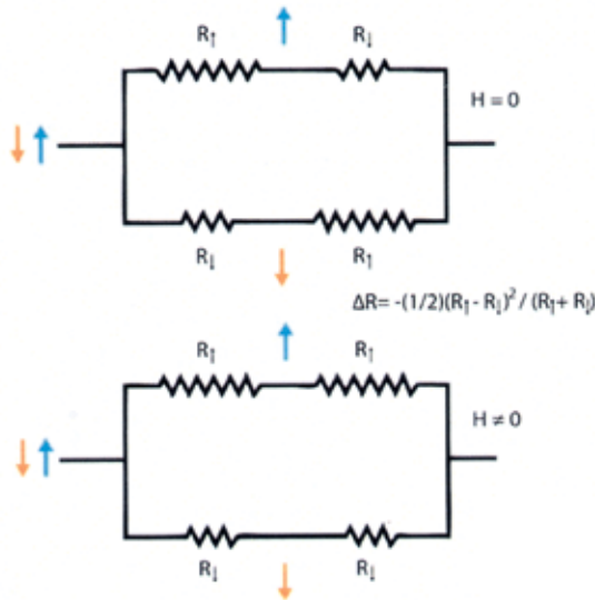
Fig. 7: The same physical system as in Fig. 6. The magnetic layers are now represented by resistances R_\uparrow and R_\downarrow . This shows very clearly that the total resistance for the two cases are different, i.e. there is a magnetoresistance effect. In case R_\uparrow \gg R_\downarrow it is practically only the lowest of the four possibilities which will permit a current. In the lower picture with parallel magnetizations the resistance for the spin up (spin down) electrons will be R_\uparrow ( R_\downarrow ) in both magnetic layers. In the upper picture with antiparallel magnetizations the spin up (spin down) electrons will have a resistance R_\uparrow ( R_\downarrow ) in the first magnetic layer to the left. In the second magnetic layer the resistance for the spin up (spin down) electron will be R_\downarrow ( R_\uparrow ), since the magnetization environment has here become totally opposite compared to the first magnetic layer.
