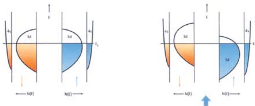
Fig. 3: To the left a schematic plot is shown for the energy band structure of a d transition metal. The density of states N(E) is shown separately for the spin up and down electrons and where a simplified separation has been made between the 4 s and 3 d band energies. For the non-magnetic state these are identical for the two spins. All energy levels below the Fermi energy are occupied states (orange and blue). The coloured area (orange + blue) corresponds to the total number of valence electrons in the metal. To the right the corresponding picture is illustrated for a ferromagnetic state, with a spin-polarization chosen to be in the up direction ( N_{\uparrow} > N_{\downarrow} ; blue area > orange area). This polarization is indicated by the thick blue arrow at the bottom figure to the right.
