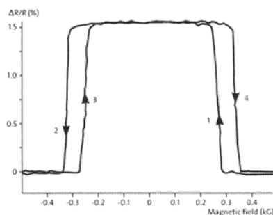
Fig. 2: After Refs. [3] and [4]. Left: Magnetoresistance measurements [3] (room temperature) for the trilayer system Fe/Cr/Fe. To the far right as well as to the far left the magnetizations of the two iron layers are both parallel to the external magnetic field. In the intermediate region the magnetizations of the two iron layers are antiparallel. The experiments also show a hysteresis behaviour (difference 1 and 4 (2 and 3)) typical for magnetization measurements. Right: Magnetoresistance measurements [4] (4.2 K), for the multilayer system (Fe/Cr) n . To the far right ( >H_S , where H_S is the saturation field) as well as to the far left ( < -H_S ) the magnetizations of all iron layers are parallel to the external magnetic field. In the low field region every second iron layer is magnetized antiparallel to the external magnetic field. 10 kG = 1 Tesla.
