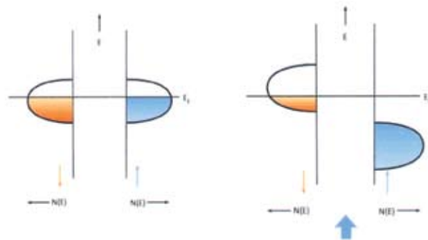
Fig. 8: Schematic illustration of the density of states for non-magnetic (left) and ferromagnetic \text{CrO}_2 (right). As can be seen immediately for the ferromagnetic case (right), the spin down electrons (orange) are placed in a metallic band, while the spin up electrons (blue) show an electronic structure that is typical for an insulator. The net spin polarization is shown by a thick blue arrow.
